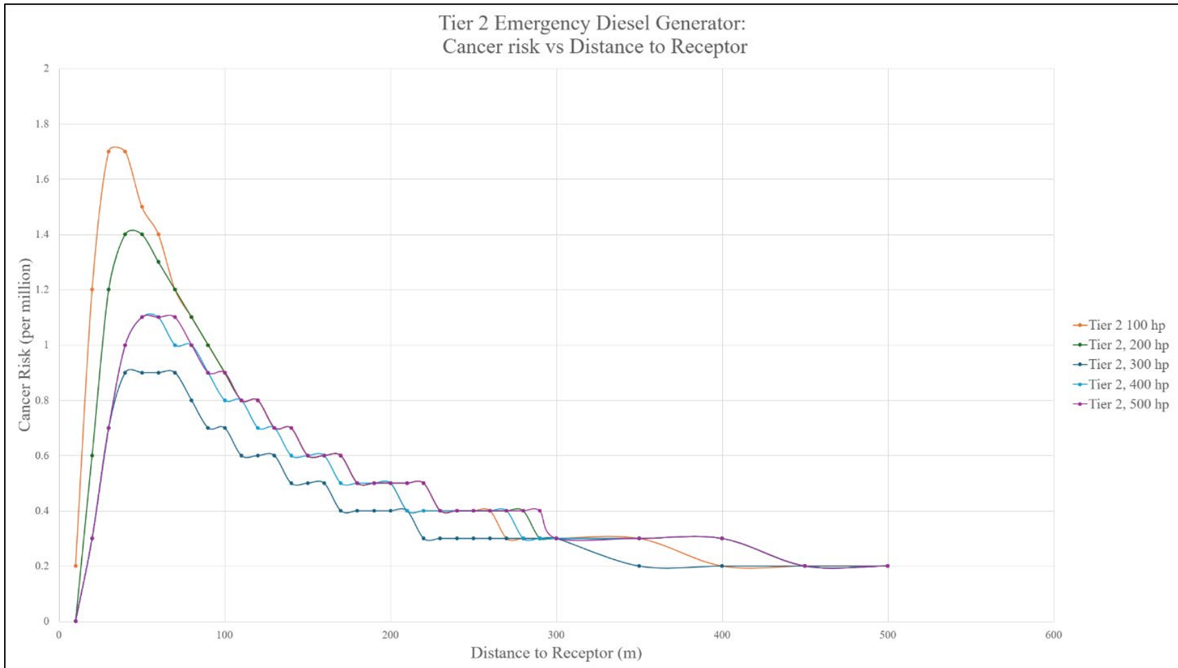
Figure 2. This graph depicts the changes in cancer risks calculated by the CARB DICE tool of tier 2 Diesel generator engines at varying color-coded horsepower vs the distance to receptors in meters.
