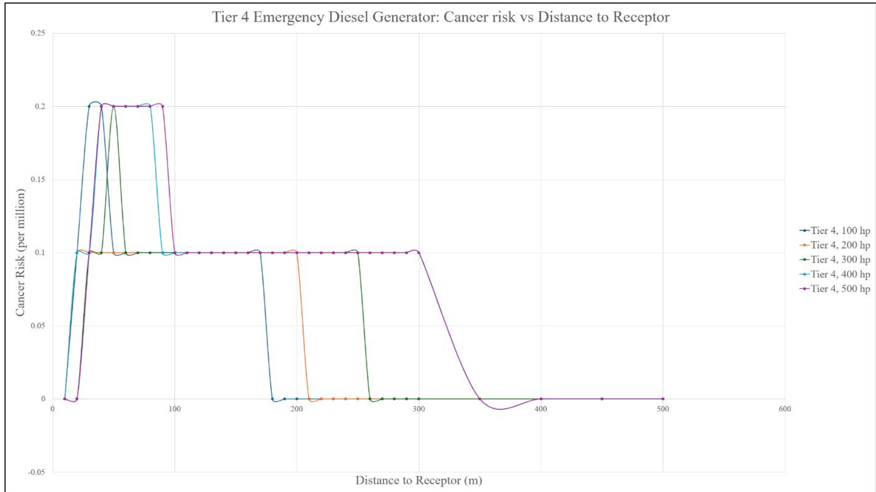
Figure 4. This graph depicts the changes in cancer risks calculated by the CARB DICE tool of tier 4 Diesel generator engines at varying color-coded horsepower vs the distance to receptors in meters.
