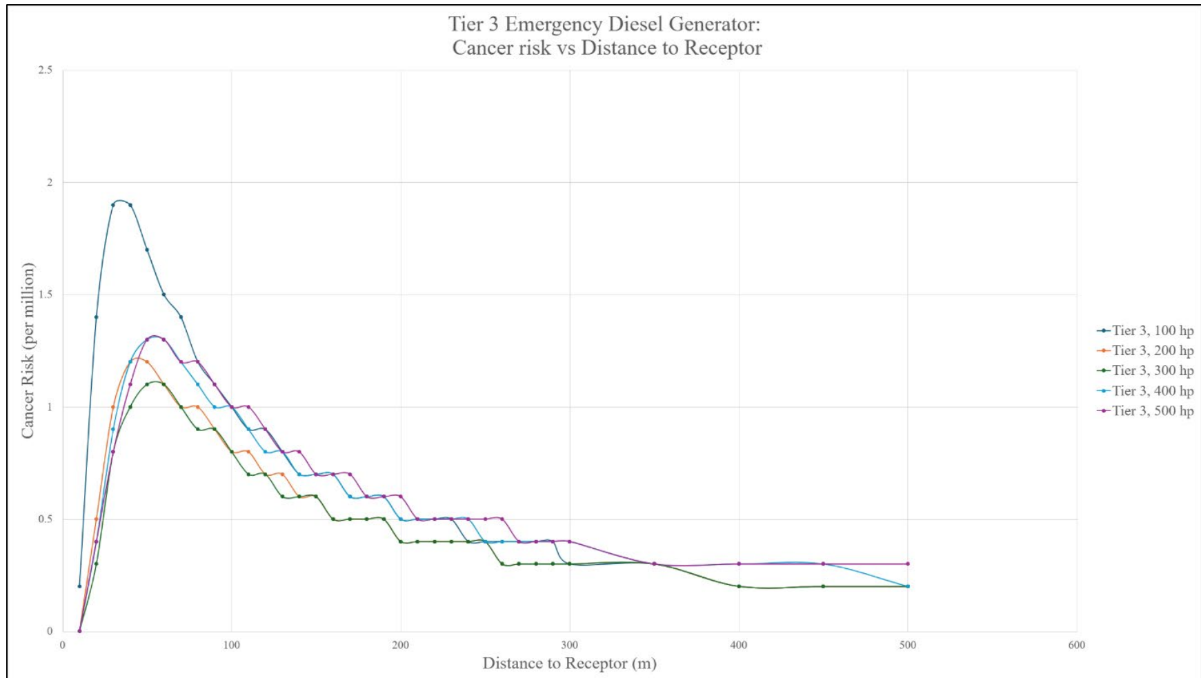
Figure 3. This graph depicts the changes in cancer risks calculated by the CARB DICE tool of tier 3 Diesel generator engines at varying color-coded horsepower vs the distance to receptors in meters.
