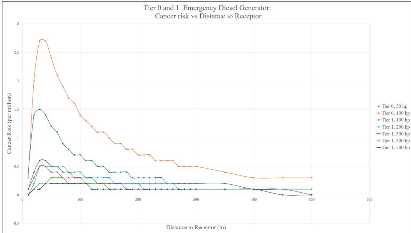
Figure 1. This line graph depicts the changes in cancer risk calculated by the CARB DICE tool of tier 0 and 1 Diesel generator engines at varying horsepower vs the distance to nearest receptor (public person outside facility) in meters. Tier 1 and 0 are the dirtiest emission tiers for diesel engines and represent worst-case scenarios.
